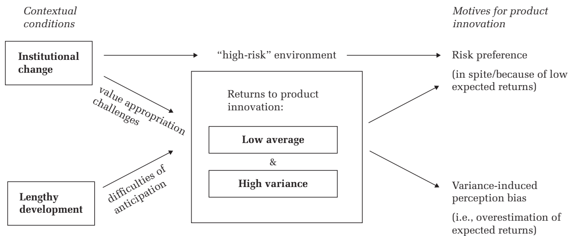
FIGURE 2 Interpretative Model
